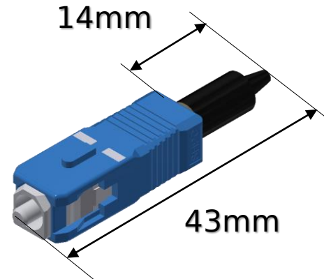
SC connector Short Boot
